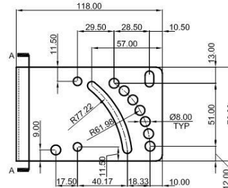
MOUNTING PLATE
