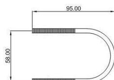
"U" BOLT
